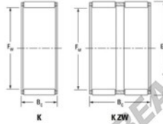
For needle roller and cage assemblies
