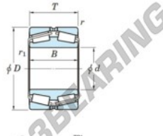
Boundary dimensions
