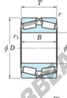
Boundary dimensions
