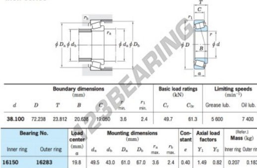
Single-row tapered roller bearings — Koyo inch series
